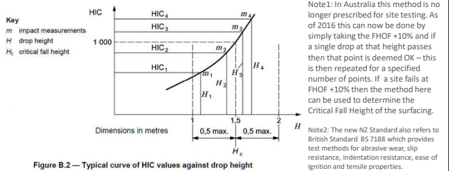
Figure B.2 — Typical curve of HIC values against drop height
