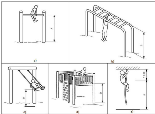
Figure 14 (part) – Examples showing Free Heights of Fall
