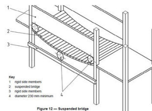
Figure 12 — Suspended bridge
