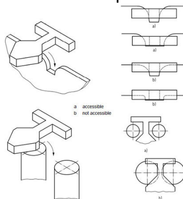
Figure D.3 — Method of insertion of the 'B' portion of the test template
