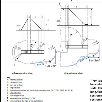
Figure 9 — Impact area of slides
