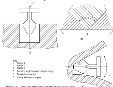
Figure D.4 — Checking all insertion angles to determine range
