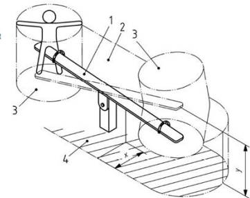
Figure 9 — Examples of falling space of rocking equipment Type 1
