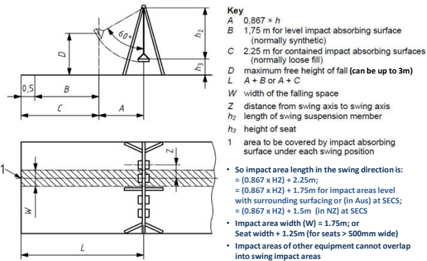
Figure 9 — Free height of fall and surfacing requirements beneath a swing
