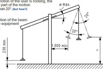
Figure 12 — Free height of fall of overhead single axis seesaw (Type 6)
