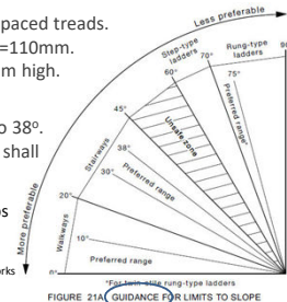
FIGURE 21A GUIDANCE FOR LIMITS TO SLOPE
