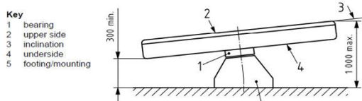
Figure 11 — Example of carousel type E (giant revolving disk) showing requirements for ground clearance
