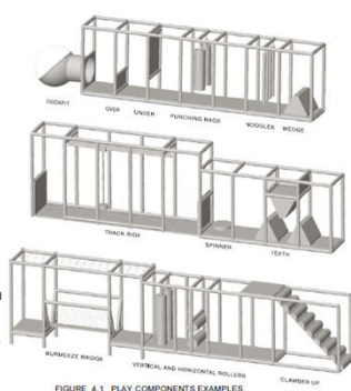
FIGURE 4.1 PLAY COMPONENTS EXAMPLES
