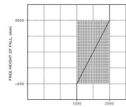
FIGURE 3.5 MINIMUM EXTENT OF FALL ZONE—OTHER CASES
