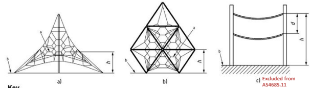
Figure 5 — Free height of fall
