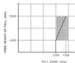
FIGURE 3.4 MINIMUM EXTENT OF FALL ZONE—TODDLER AREAS
